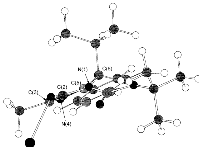
Figure 2. Molecular mechanics calculations of potassium enolate of 2
