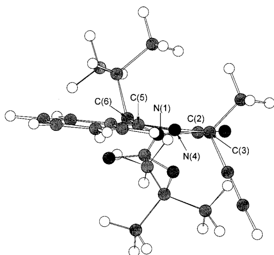
Figure 3. Molecular mechanics calculations of compound (6R)-6c
