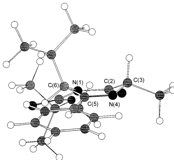
Figure 1. Molecular mechanics calculations of 2-pyrazinone 2
